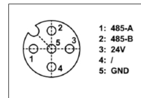
M12-5Connector
