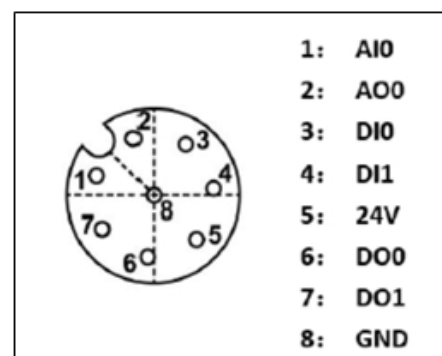
M12-8Connector
